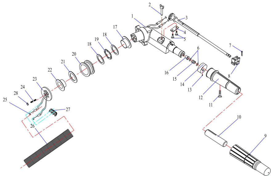
Tiller Handle
