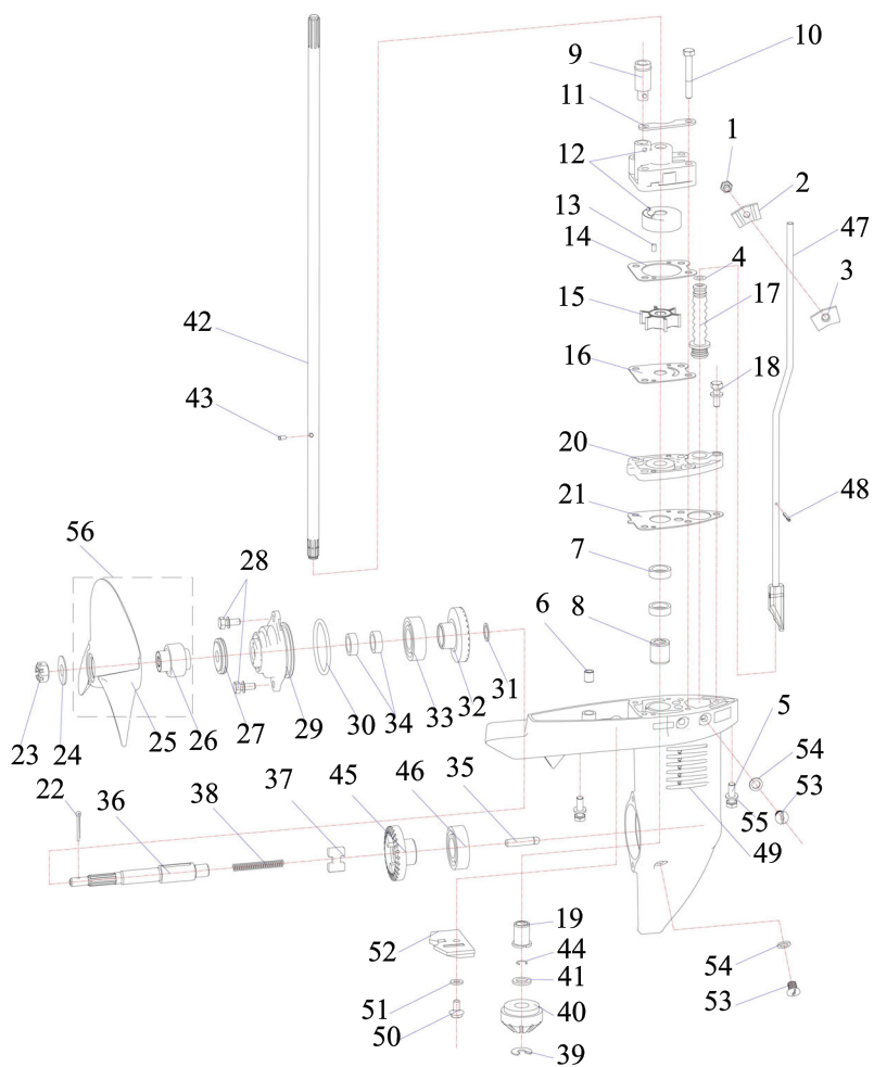
Lower units
