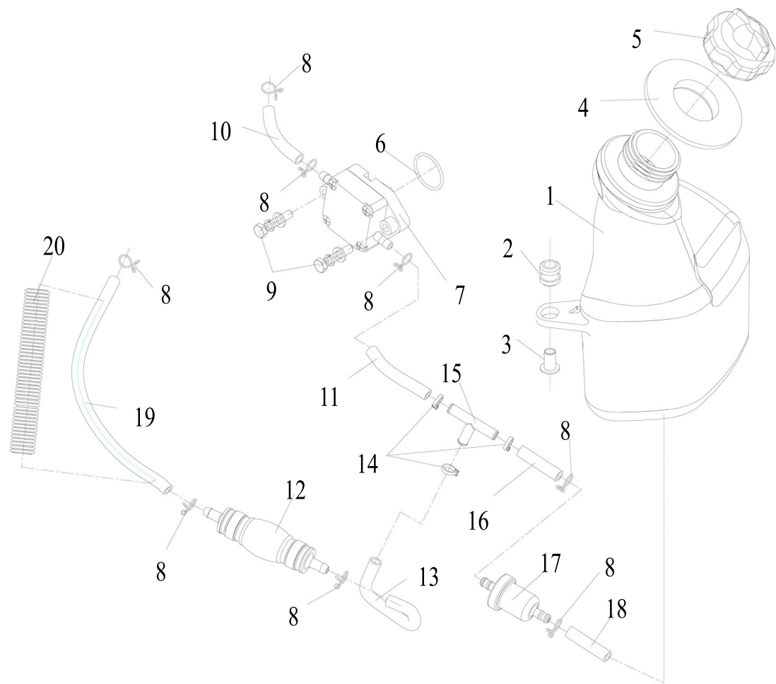
Fuel system
