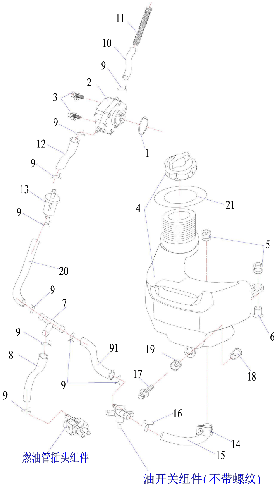
Fuel system
