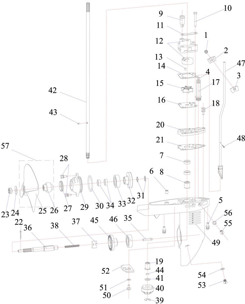
Lower units
